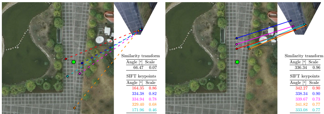
(c) Without orientation and scale check (d) With orientation check, with/without scale check
