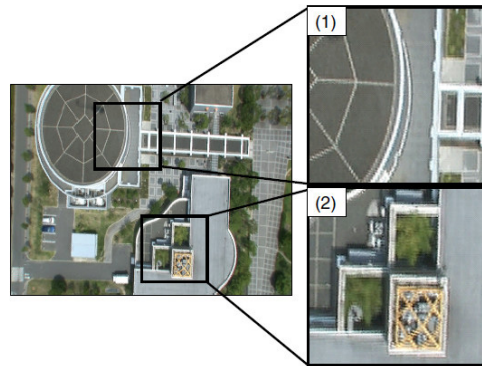
Super-resolved image
