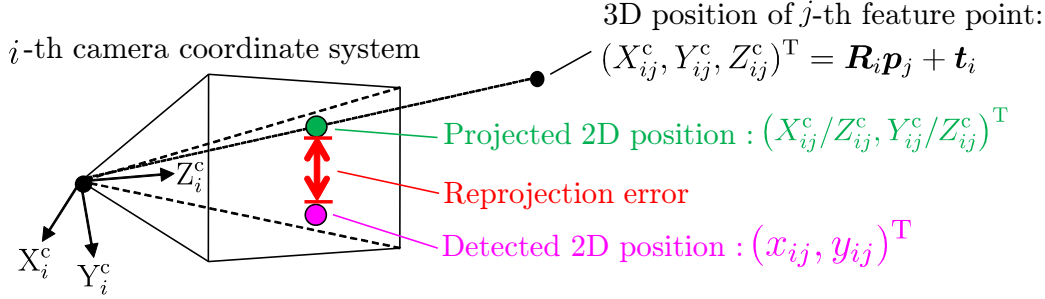
Figure 2.2: Reprojection error.
