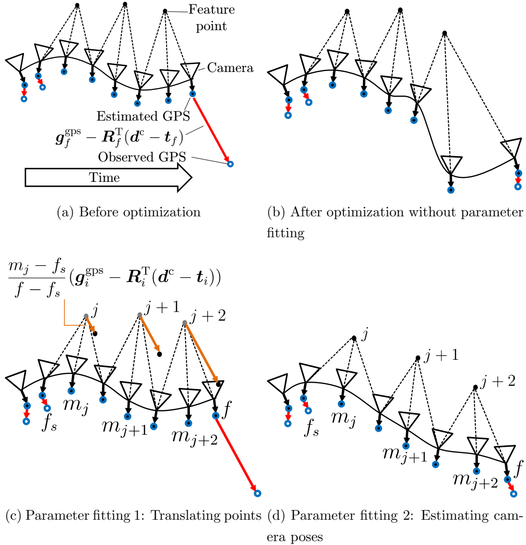
Figure 2.4: Parameter fitting to GPS positions.
