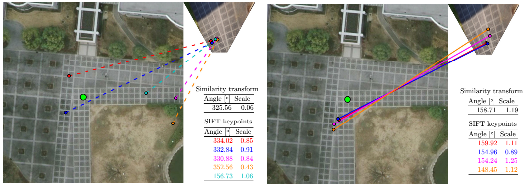
(a) Without orientation and scale check (b) With scale check, with/without orientation check
